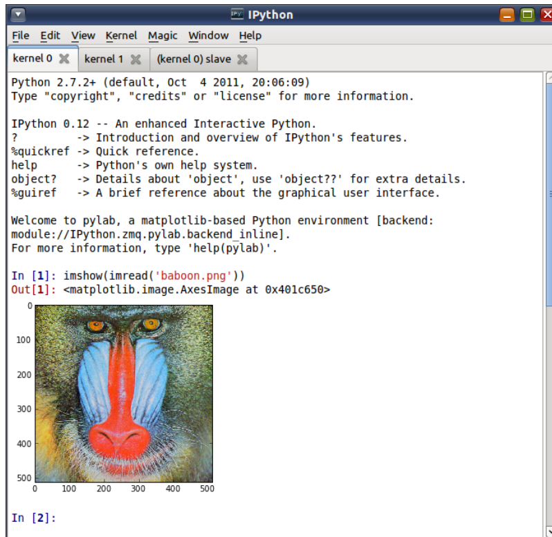
Fig. 4: The improved Qt console for IPython, now with tabs to control multiple kernels and full menu support.
